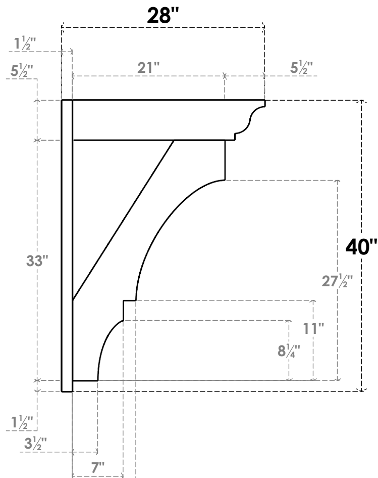
SIDE PROFILE
